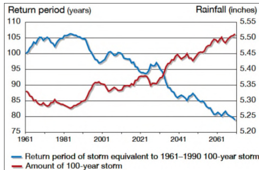
Figure 5.4.6-1. Projected Rainfall and Frequency of Extreme Storms
